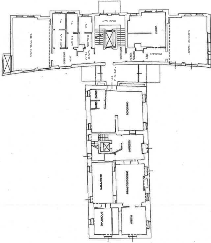
PIANO TERRA H: 2,90 m
